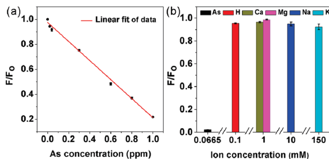
Figure 1. (a) Linear relation between the relative emission intensity of nanoprobe ( F/F_0 ) and the concentration of arsenic. The concentration of As is from 0.02 to 1 ppm, the F/F_0 is from 0 to 1, and the nanoprobe concentration is fixed at 250 nM. (b) The relative emission intensity of nanoprobe when they are incubated with different metal ions, respectively, the K + is at 150 mM, Na + is at 10 mM, Ca 2+ and Mg 2+ are at 1 mM, H + is at 0.1 mM, and As is at 0.0665 mM, representing concentrations as found in a live cell. 13,14,25–28 The nanoprobe concentration is fixed at 250 nM in all studies. This result revealed that only arsenite could specifically decrease the emission intensity of the nanoprobe.
